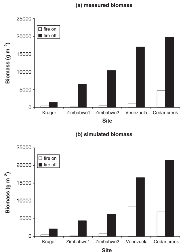
Fig. 1 Above-ground woody biomass in savannas with 'fire on' (burnt every 2–3 yr) and 'fire off' (unburnt for 40+ yr). (a) Measured biomass in g m -2 dry weight; (b) simulated biomass using the Sheffield Dynamic Global Vegetation Model (SDGVM; maximum values for fire off, median values for fire on). Sites are Kruger National Park (Shackleton & Scholes, 2000); Zimbabwe 1, Matopos (Kennan, 1972, P. Frost pers. comm., 2003), Zimbabwe 2, Marondera (Barnes, 1965; Tsvuura, 1998, and P. Frost pers comm., 2003); Venezuela (San Jose et al. , 1998); Cedar Creek, USA (Tilman et al. , 2000).
